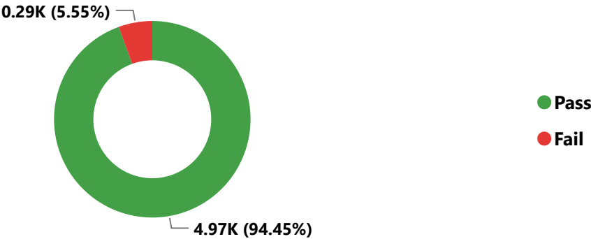
Pass/Fail Distribution
